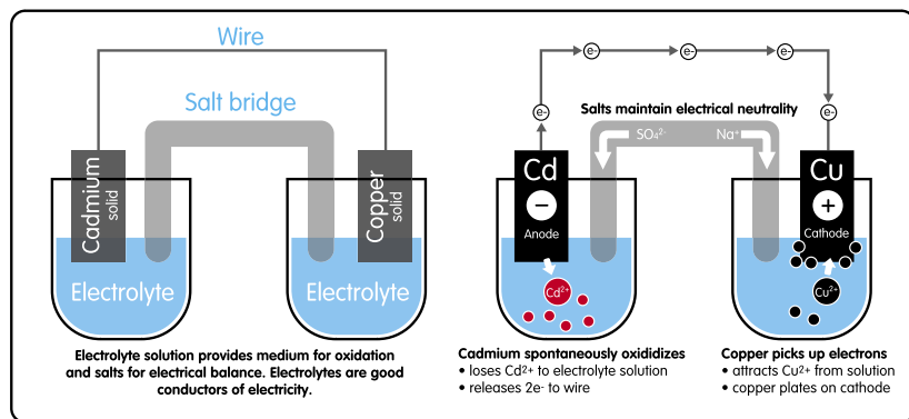
GALVANIC CELL USING THE SPONTANEOUS REDUCTION OF \text{Cu}^{2+} BY Cd TO GENERATE AN ELECTRIC CURRENT.
